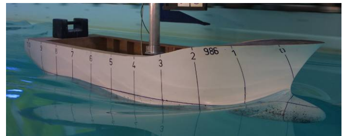
Figure 4 Design B, Depart Port Condition at 9 knots
